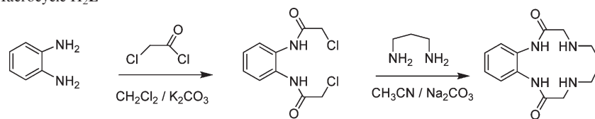
Scheme 1. Synthesis of Macrocycle H 2 L
