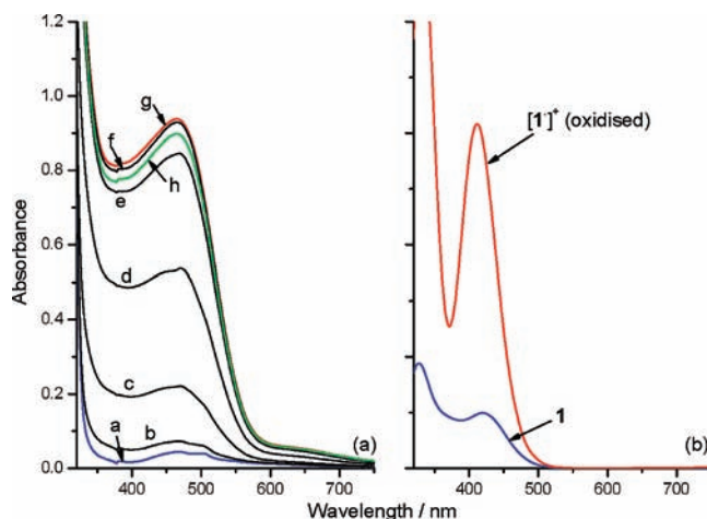
Figure 4. (a) Change observed in the experimental UV/vis absorption spectrum after in situ electrochemical oxidation of a solution of 1 ( 1.0 \times 10^{-3} M) in anhydrous, degassed DMF ( E_{\text{appl.}} = 1.13 \text{ V} , a = 0 \text{ s} , b = 40 \text{ s} , c = 108 \text{ s} , d = 212 \text{ s} , e = 317 \text{ s} , f = 420 \text{ s} , g = 733 \text{ s} , h = 1200 \text{ s} ) and, (b) simulated TD-DFT electronic absorption spectra of the 1 (blue) and the cationic triplet species, [\mathbf{1}]^+ (red).
