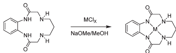
Scheme 2. Metallation of H 2 L
