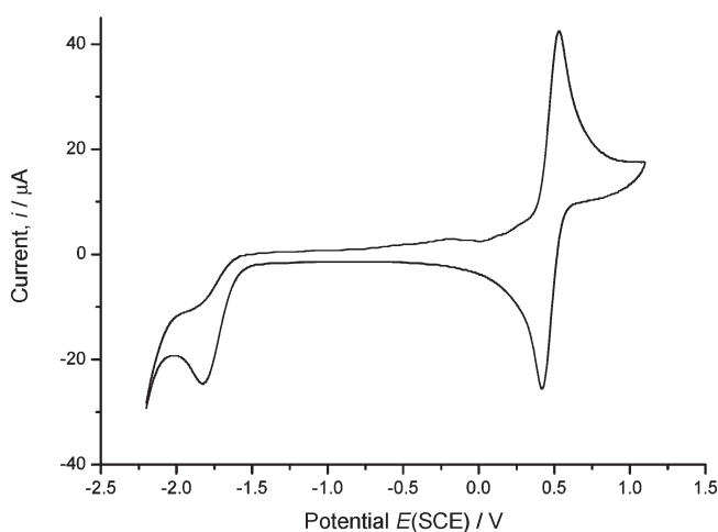
Figure 3. Cyclic voltammogram of a solution of 1 ( 5.0 \times 10^{-3} M, 22 °C) in anhydrous DMF recorded at 200 mV s -1 with n Bu 4 NBF 4 (0.10 M) supporting electrolyte recorded using a platinum disk electrode.
