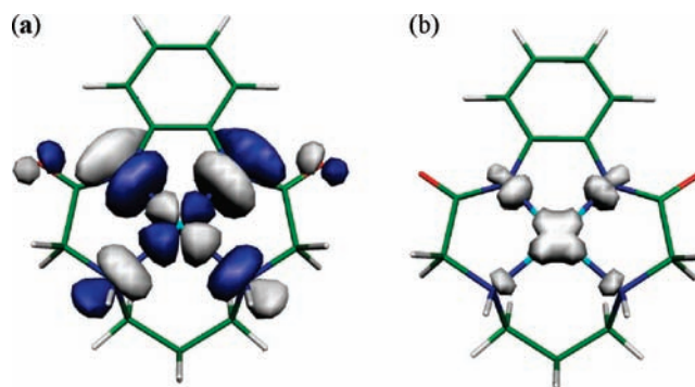
Figure 6. (a) Spatial distribution of the unoccupied \beta -LUMO orbital of 1 . The \alpha -spin spatial counterpart is the \alpha -HOMO-2 orbital in which the unpaired electron resides, and this orbital electron density correlates with the location of the calculated Mulliken spin densities. (b) Isosurface representation of the total Mulliken spin density calculated by using the molecular orbital coefficients and mapped onto the optimized structure of 1 . In-plane delocalization of spin density on to the four nitrogen donor atoms can be seen.
